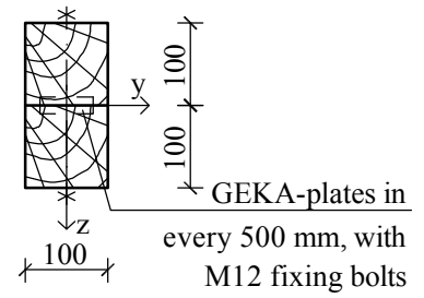
cross-section BC:
