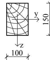
cross-section BC:
