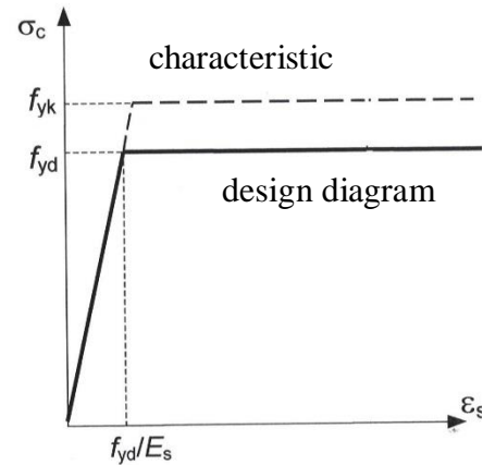
b) linear elastic- perfectly elastic
