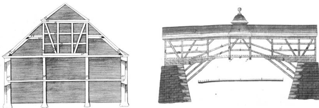
a. Stiffening measure in a roof (Vogel 1708) b. Truss Frame in a Bridge (Walter 1704) Figure 2. Craftsmanship-based structures with intuitive and traditional use of elements.
